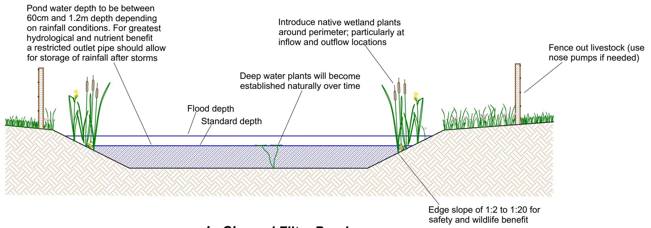
In-Channel Filter Pond
