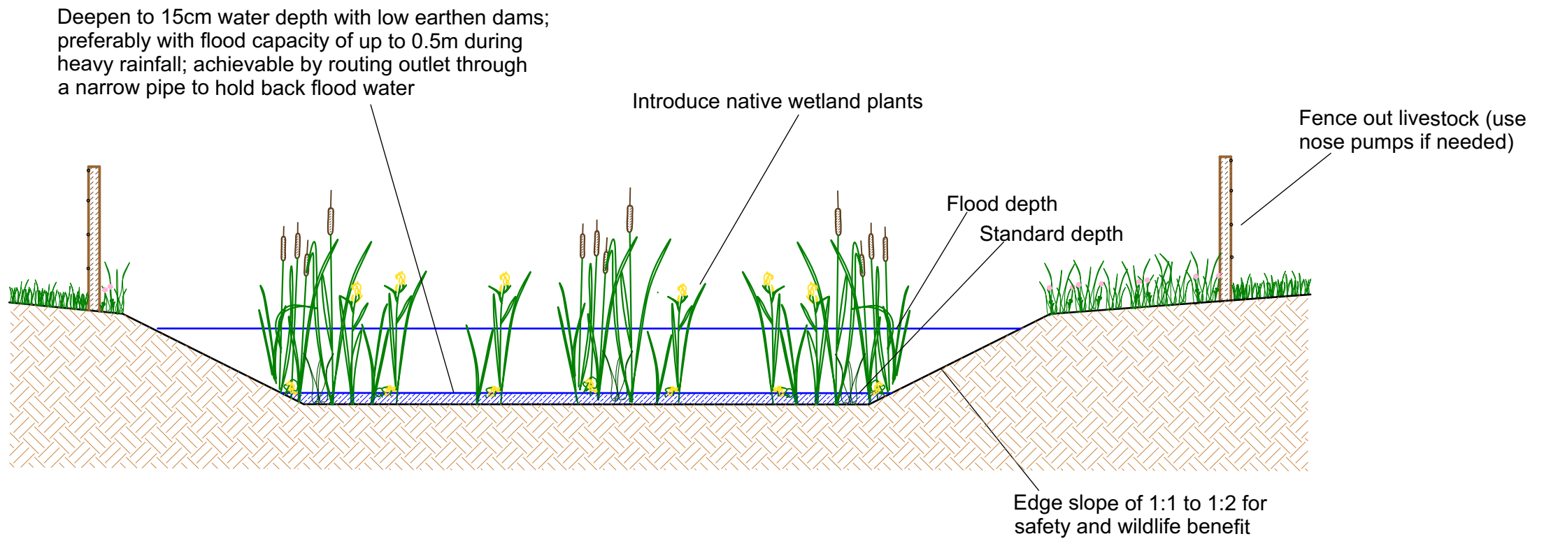
In-Channel Filter Wetland
